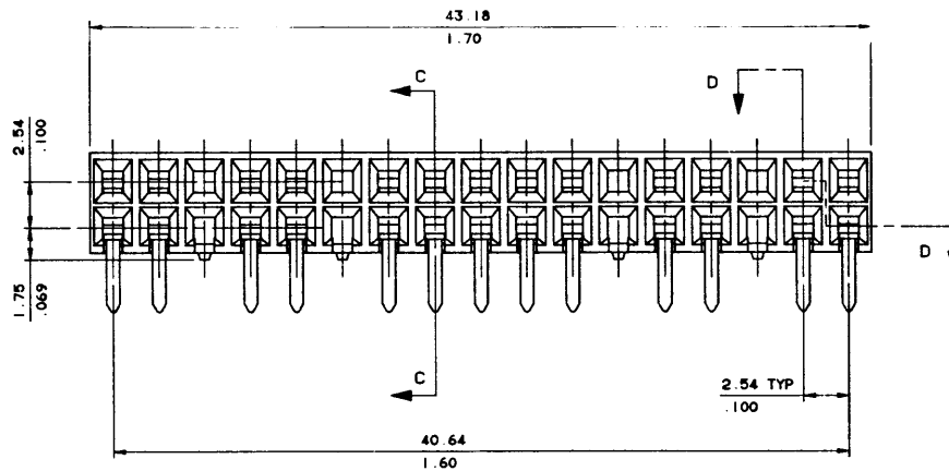
VIEW A
