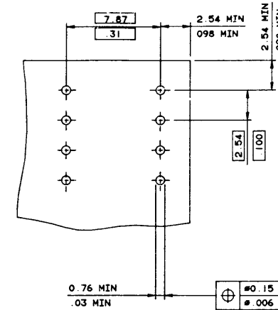
RECOMMENDED HOLE PATTERN
