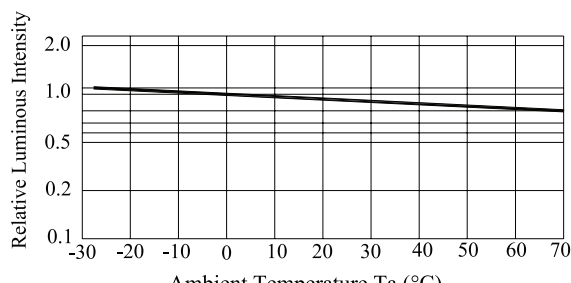
Fig.6 LUMINOUS INTENSITY VS. AMBIENT TEMPERATURE
