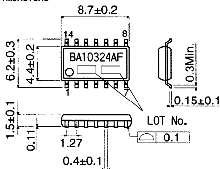
BA10324AF(SOP14) (Unit:[mm])
