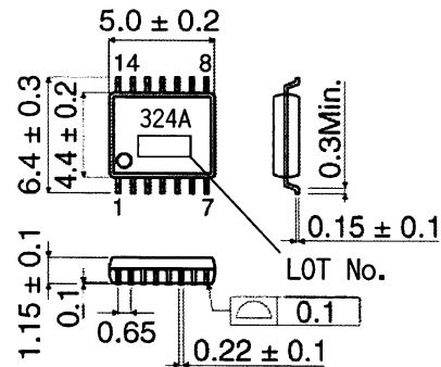
BA10324AFV(SSOP-B14) (Unit:[mm])
