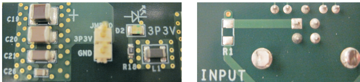
Figure 4. SN65LVPE502CP EVM location of L1, R1, and JMP10
