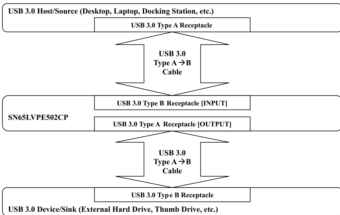
Figure 1. SN65LVPE502CP Functional System Level Block Diagram
