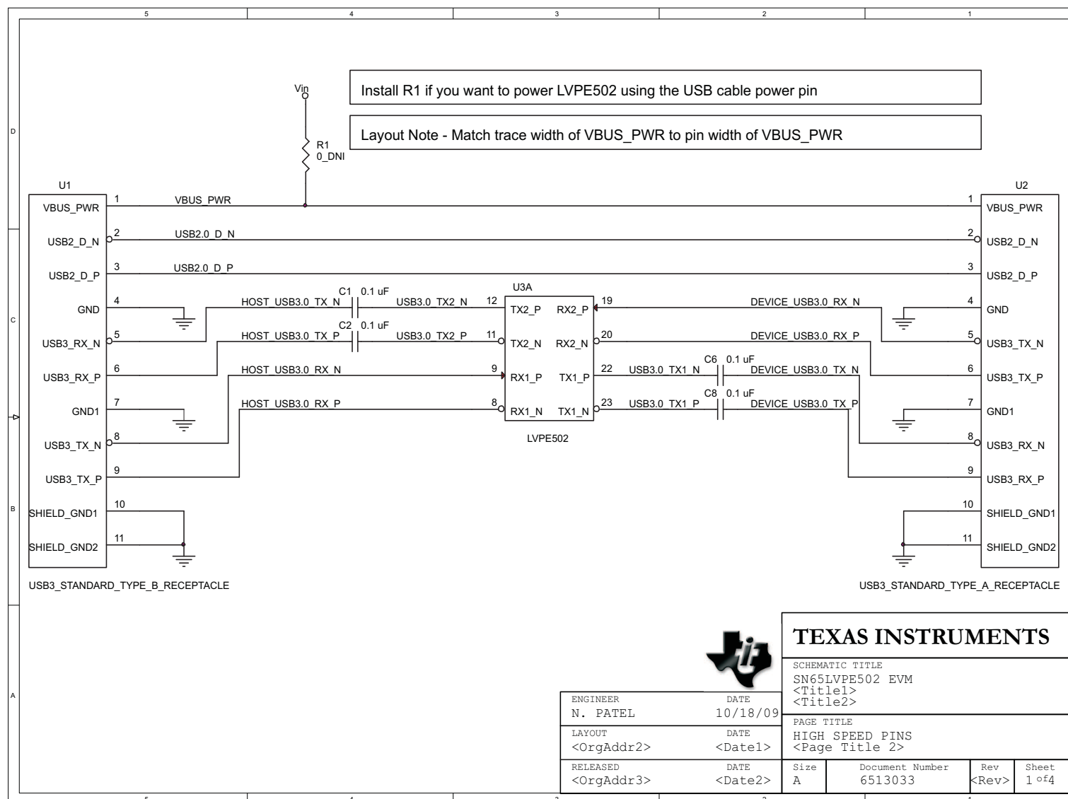
Figure 5. SN65LVPE502CP EVM Schematic (High Speed Pins)
