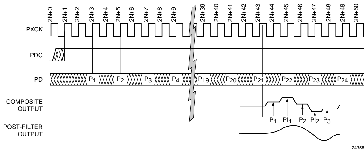
Figure 17. External Pixel Data Control
