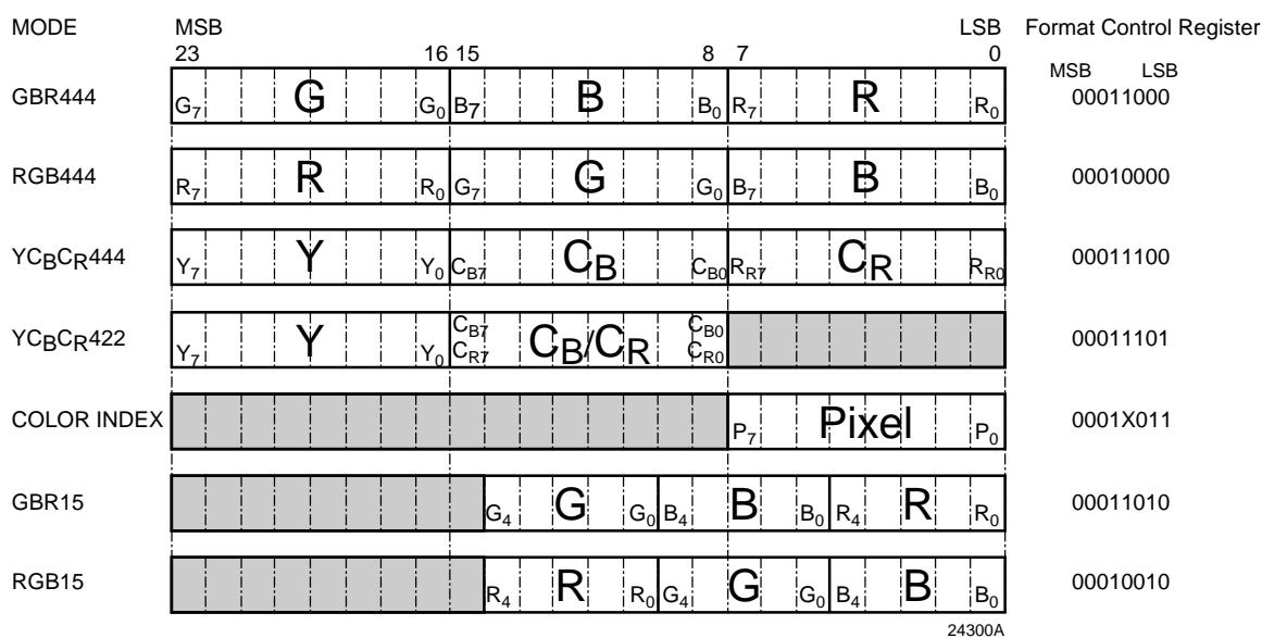
Figure 1a. Pixel Data Format
