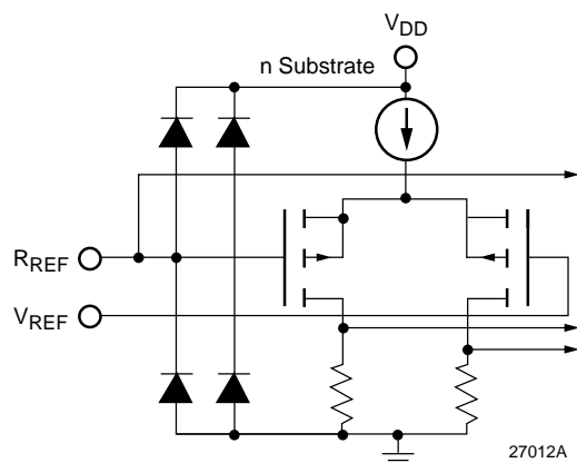
Figure 30. Equivalent Analog Input Circuit
