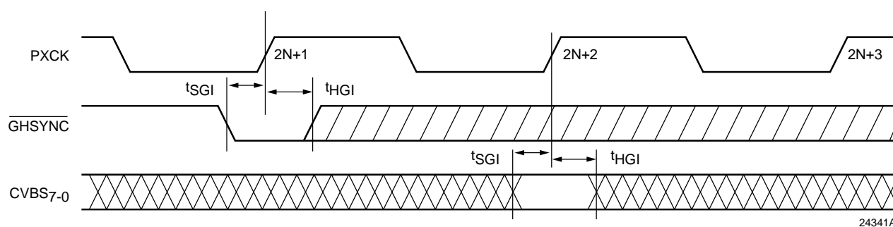
Figure 24. Genlock Interface Timing
