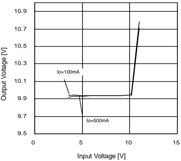
Figure 24. Line Regulation
