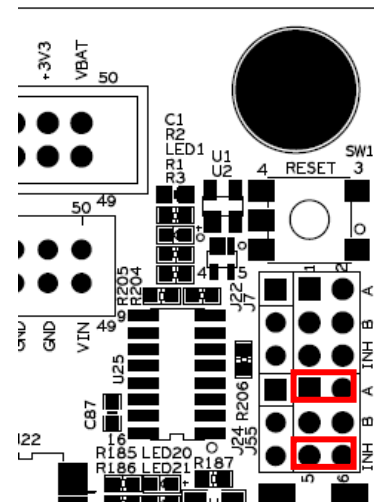
Figure 34 – Jumper Setting: PIO1_11, SSEL to Dataflash, U15
