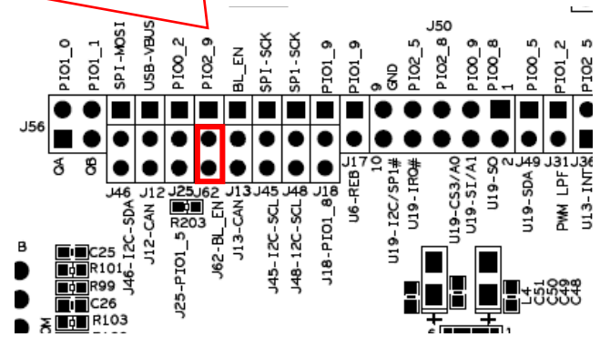
Figure 43 – Jumper Setting: J62 and BL-button
