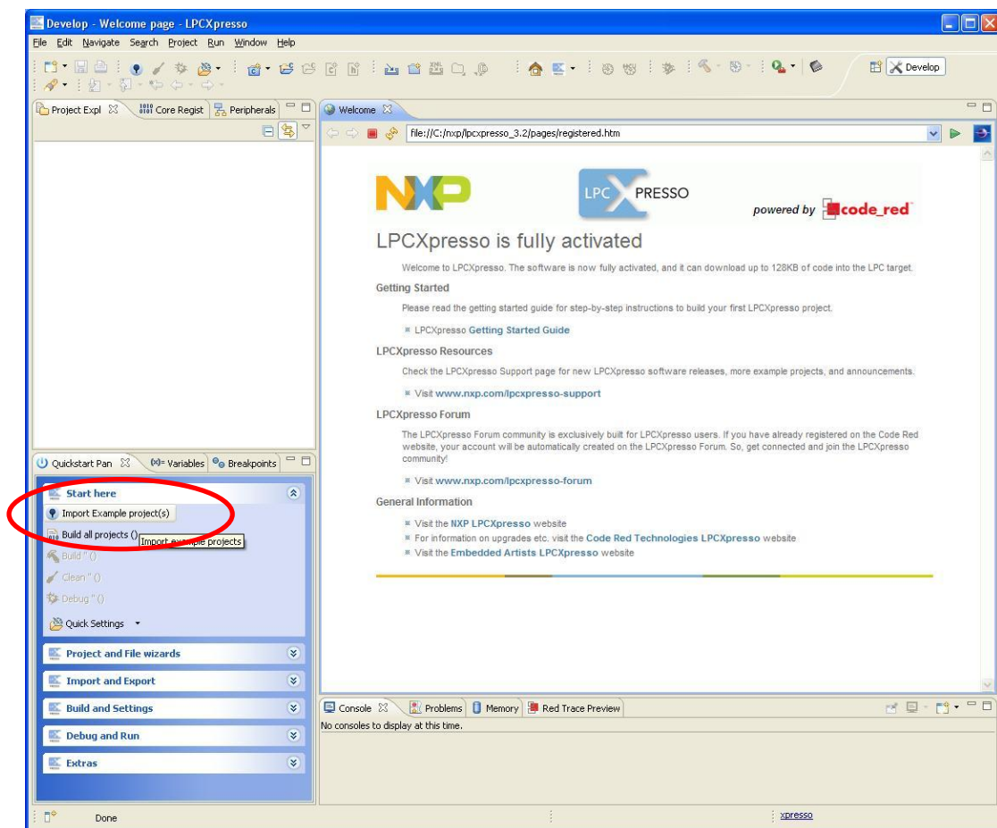
Figure 11 – Import project
