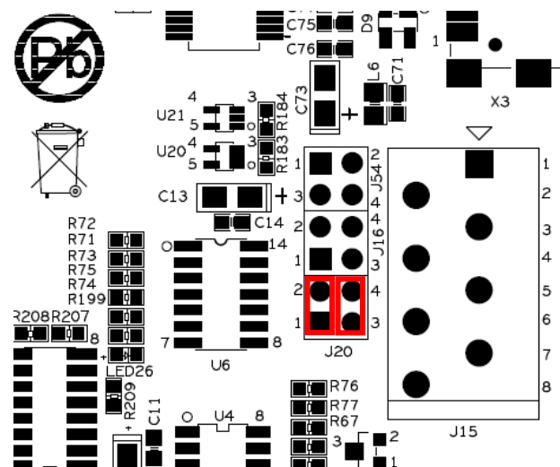
Figure 25 – Jumper Setting: Rs422 termination
