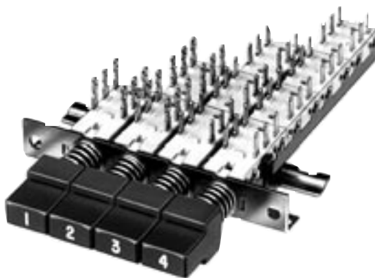
SERIES 90000 with A-650 Pushbuttons Installed
