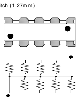
745X102 8 Resistors 10 Terminations
