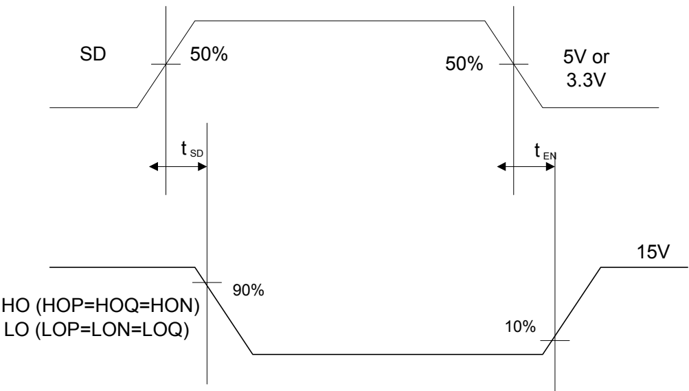
Figure 10 Shutdown Timing
