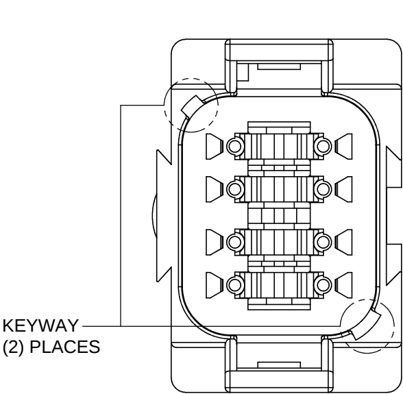
P/N AT04-08PC KEY-C CONFIGURATION STANDARD COLOR: GREEN
