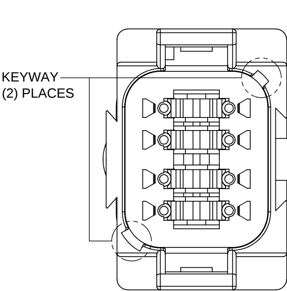
P/N AT04-08PD KEY-D CONFIGURATION STANDARD COLOR: BROWN
