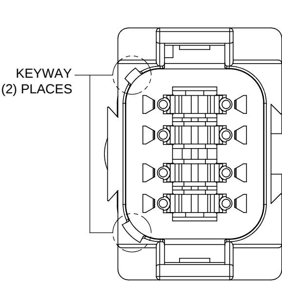
P/N AT04-08P KEY-A CONFIGURATION STANDARD COLOR: GREY
