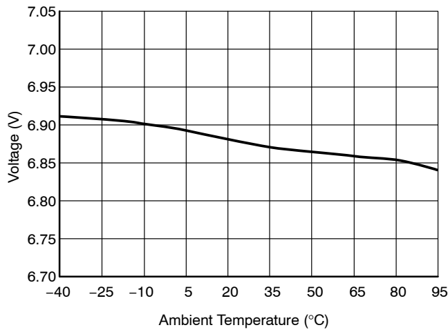
Figure 24. Typical V_{th} Threshold Variation vs. Temperature
