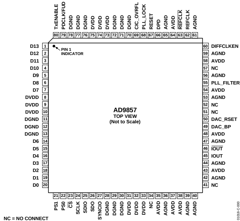
Figure 2. Pin Configuration
