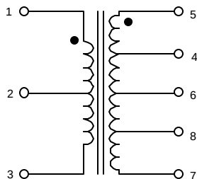
SCHEMATIC "4"
