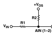
Figure 12. Scaling and Offsetting AIN(1-2) for Negative Inputs
