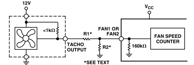
Figure 17d. Fan with Strong Tach. Pull-Up to >V CC or Totem-Pole Output, Attenuated with R1/R2
