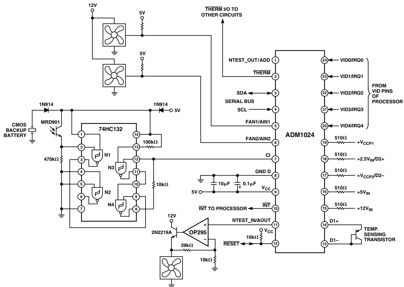
Figure 25. Application Circuit
