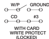
Part Nos. Available SDP-09-SG-A (Normal Type, No Standoff) SDP-09-SG-B (Normal Type, 1.5mm Standoff) SDP-09-SG-C (Normal Type, 1.8mm Standoff) SDP-09-SG-D (Normal Type, 2.2mm Standoff) SDPR-09-SG-A (Reverse Type, No Standoff)
