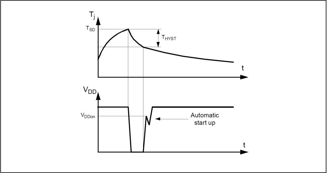
Figure 13. Thermal shutdown
