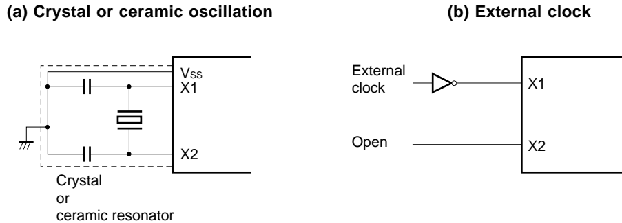
Figure 6-3. External Circuit of System Clock Oscillator
