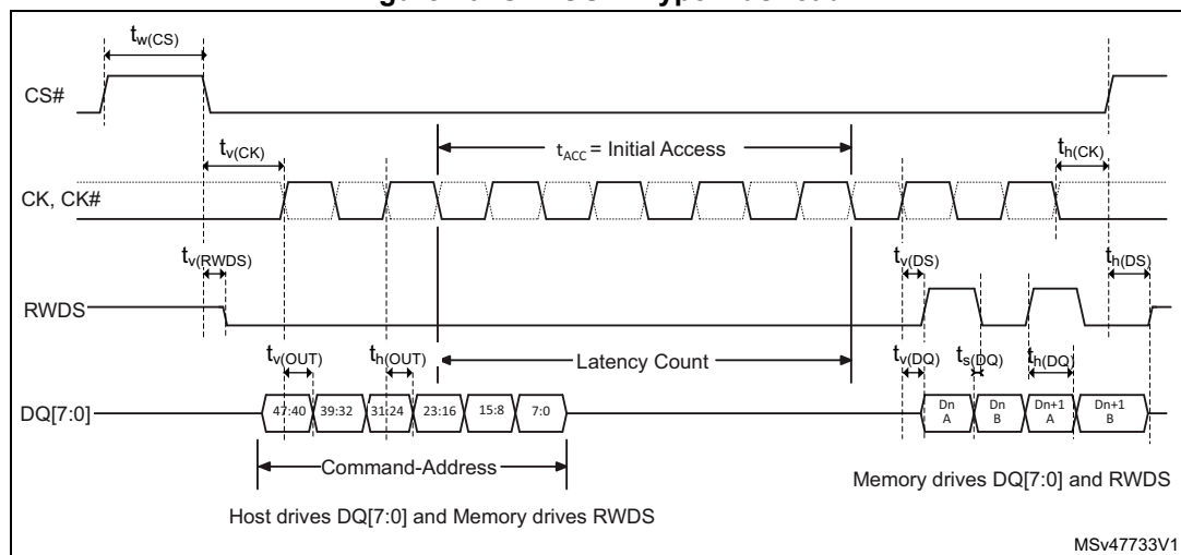
Figure 70. OCTOSPI HyperBus read
