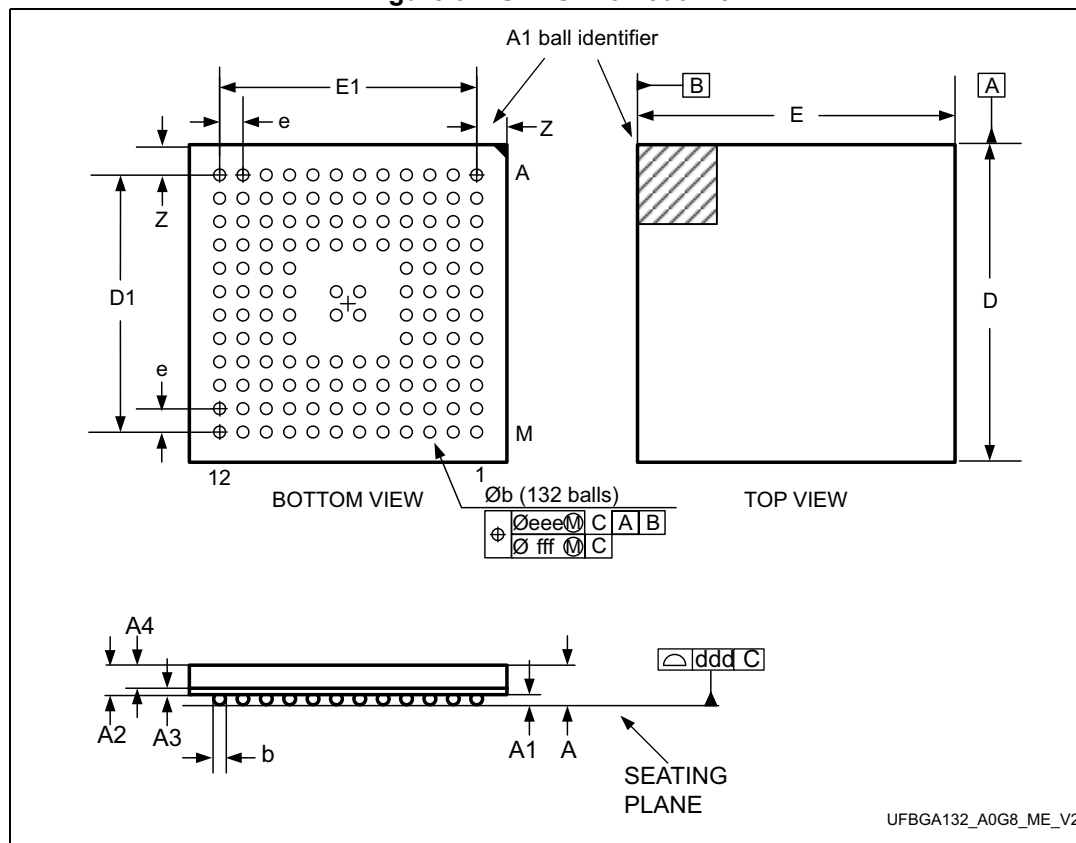
Figure 91. UFBGA132 outline
