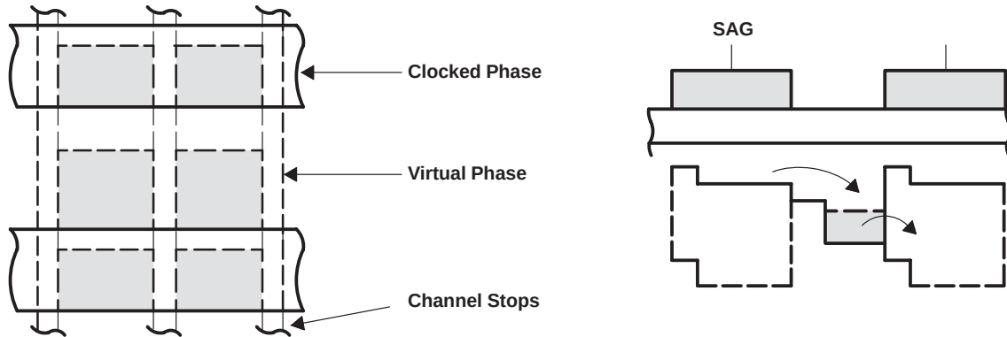
Figure 2. Charge-Transfer Process
