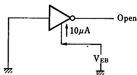
Test Circuit 3 ( V_{EB} )
