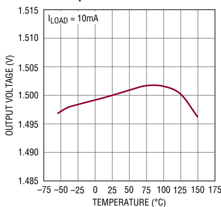
Output Voltage (1.5V) vs Temperature
