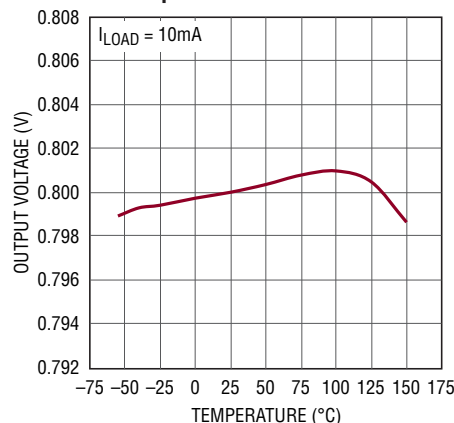
Output Voltage (0.8V) vs Temperature
