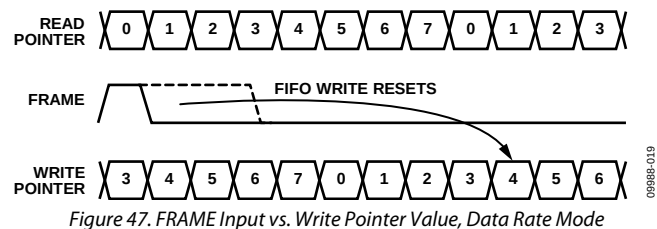
Figure 47. FRAME Input vs. Write Pointer Value, Data Rate Mode
