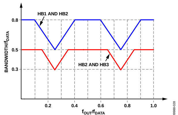
Figure 57. Signal Bandwidth vs. Center Frequency of the Output Signal, 4x Interpolation
