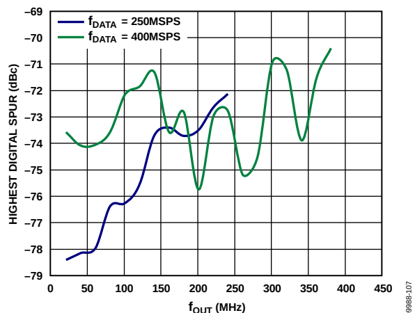
Figure 10. Highest Digital Spur vs. f_{OUT} over f_{DATA} , 2x Interpolation, Digital Scale = 0 dBFS, I_{FS} = 20 mA
