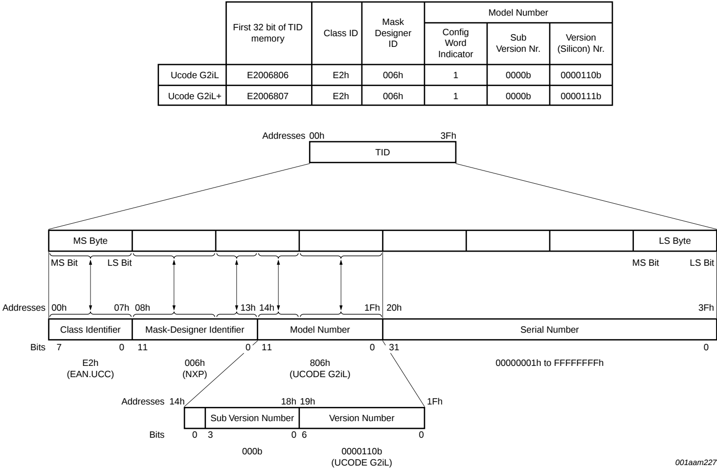
Fig 6. G2iL TID memory structure
