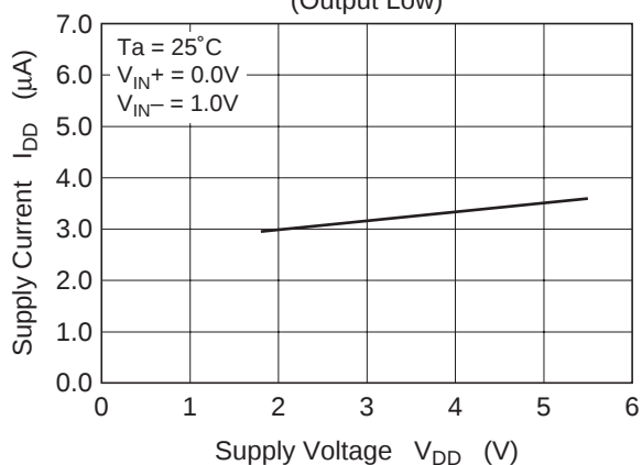
Figure 3-2 HA1631S03 Supply Current vs. Supply Voltage (Output Low)
