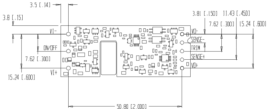
Bottom View
