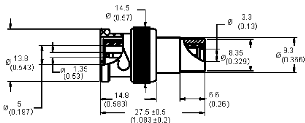
DIM OUTLINE
