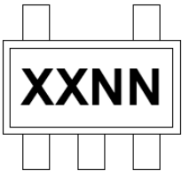
5-Lead SOT-23 (MCP6546, MCP6546R, MCP6546U)
