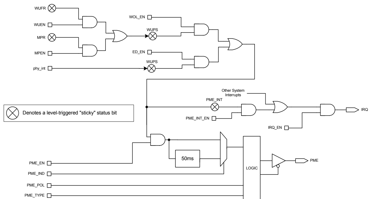
Figure 3.18 PME and PME_INT Signal Generation
