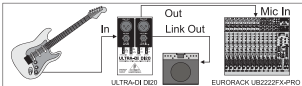
Fig. 2.1: Guitar ➡ DI-box ➡ guitar amp/mixing console
