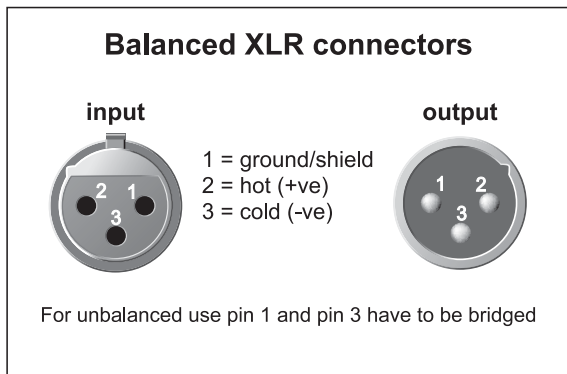
Fig. 3.1: XLR connectors
