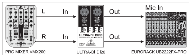
Fig. 2.2: DJ-mixer ➡ DI-box ➡ mixing console
