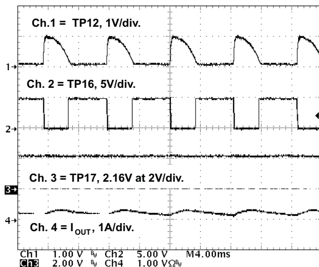
Figure 27. Triac Dimming Detection Signals, V_{IN} = 115 \text{ VAC} , f_{LINE} = 60 \text{ Hz} , V_{OUT} = 29.54 \text{ V} , I_{OUT} = 0.266 \text{ A} , (dimmer set at mid-range dimming position)
