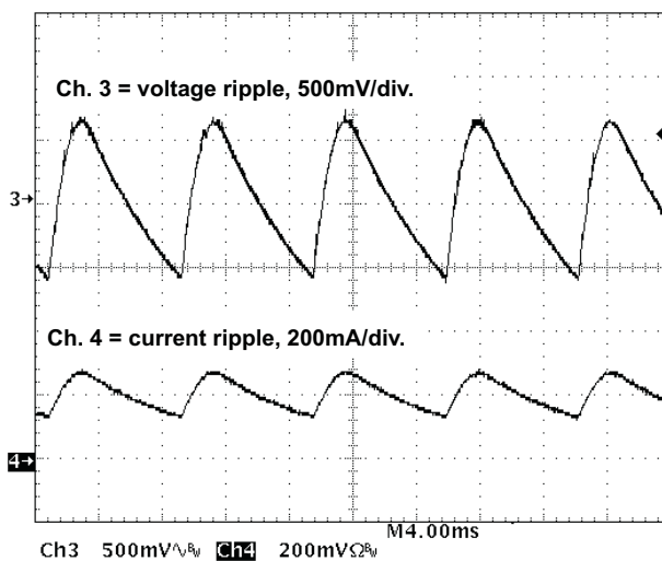
Figure 20. Output Voltage and Current Ripple, V_{\text{IN}} = 115 \text{ VAC} , f_{\text{LINE}} = 60 \text{ Hz} , Dimmer Set at Mid-Range Dimming Position, V_{\text{OUT}} = 29.41 \text{ V} , I_{\text{OUT}} = 0.228 \text{ A}
