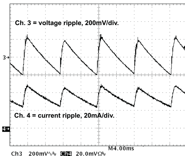
Figure 21. Output Voltage and Current Ripple, V_{\text{IN}} = 115 \text{ VAC} , f_{\text{LINE}} = 60 \text{ Hz} , Dimmer Set at Maximum Dimming Position, V_{\text{OUT}} = 27.55 \text{ V} , I_{\text{OUT}} = 0.058 \text{ A}
