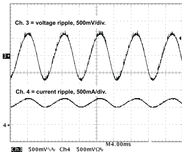
Figure 19. Output Voltage and Current Ripple, V_{\text{IN}} = 115 \text{ VAC} , f_{\text{LINE}} = 60 \text{ Hz} , No Dimmer, V_{\text{OUT}} = 31.68 \text{ V} , I_{\text{OUT}} = 0.655 \text{ A}
