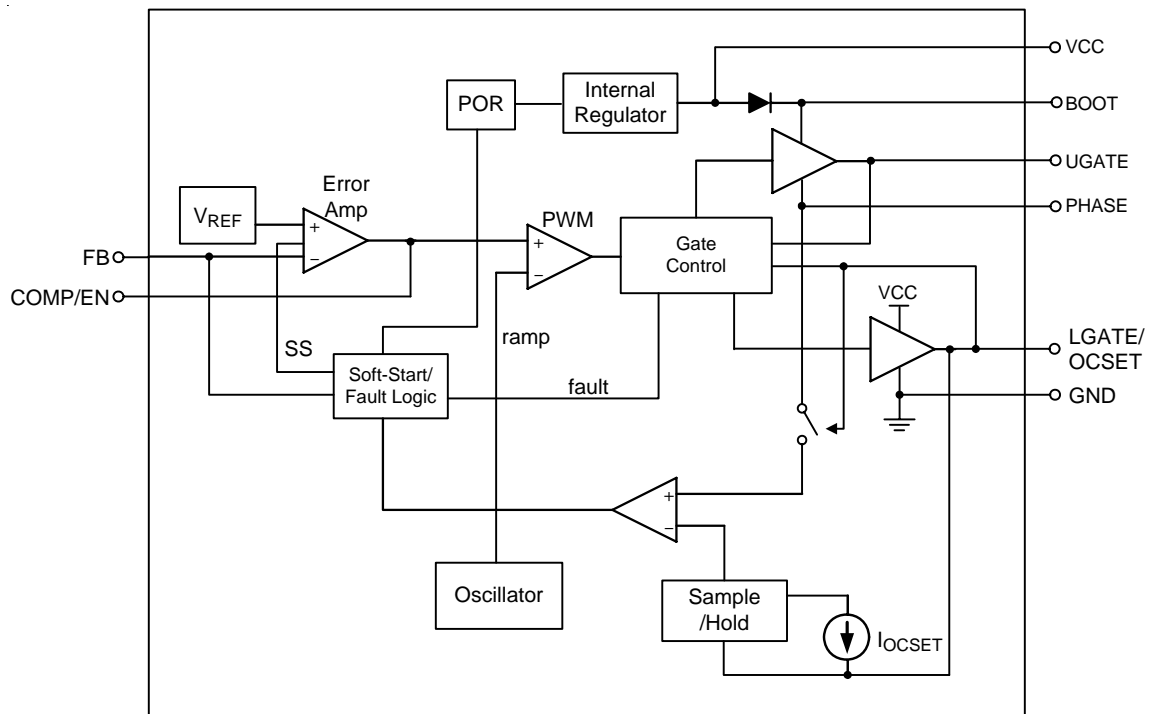
Figure 1. RT8120A/B Function Block Diagram
