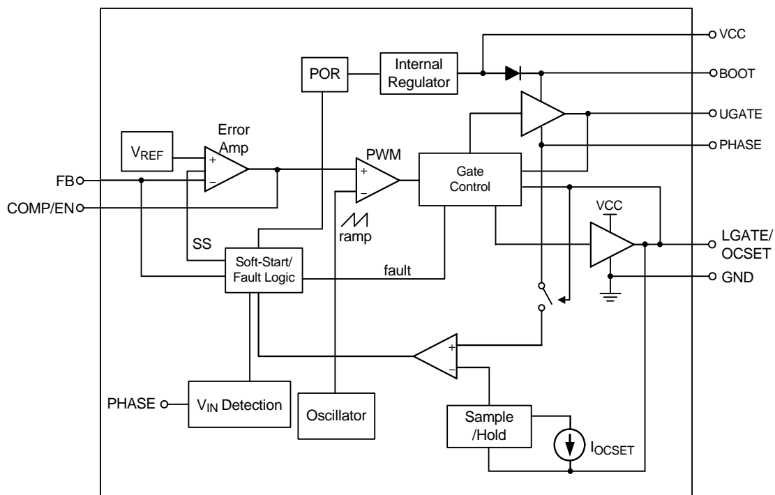
Figure 2. RT8120C/D Function Block Diagram
