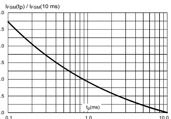
Figure 12. Relative variation of non-repetitive peak surge forward current versus pulse duration (sinusoidal waveform)
