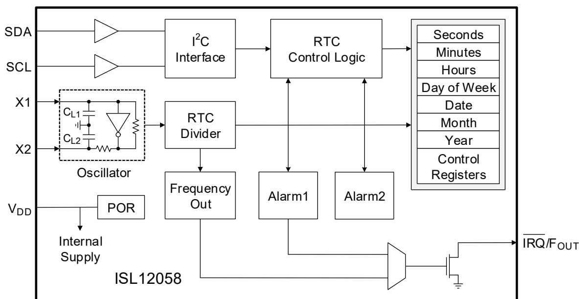
FIGURE 3. BLOCK DIAGRAM
