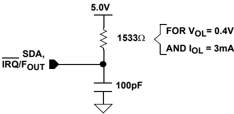
FIGURE 4. STANDARD OUTPUT LOAD FOR TESTING THE DEVICE WITH V_{\text{DD}} = 3.0\text{V} , V_{\text{PULLUP}} = 5.0\text{V}
