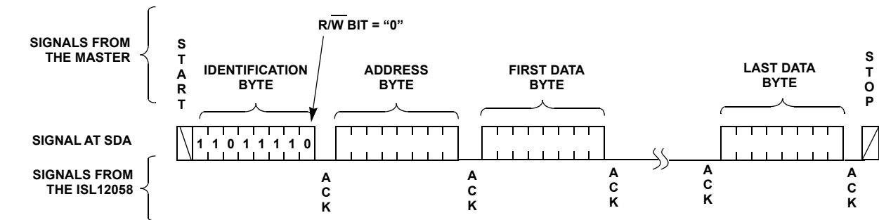
FIGURE 12. SEQUENTIAL BYTE WRITE SEQUENCE
