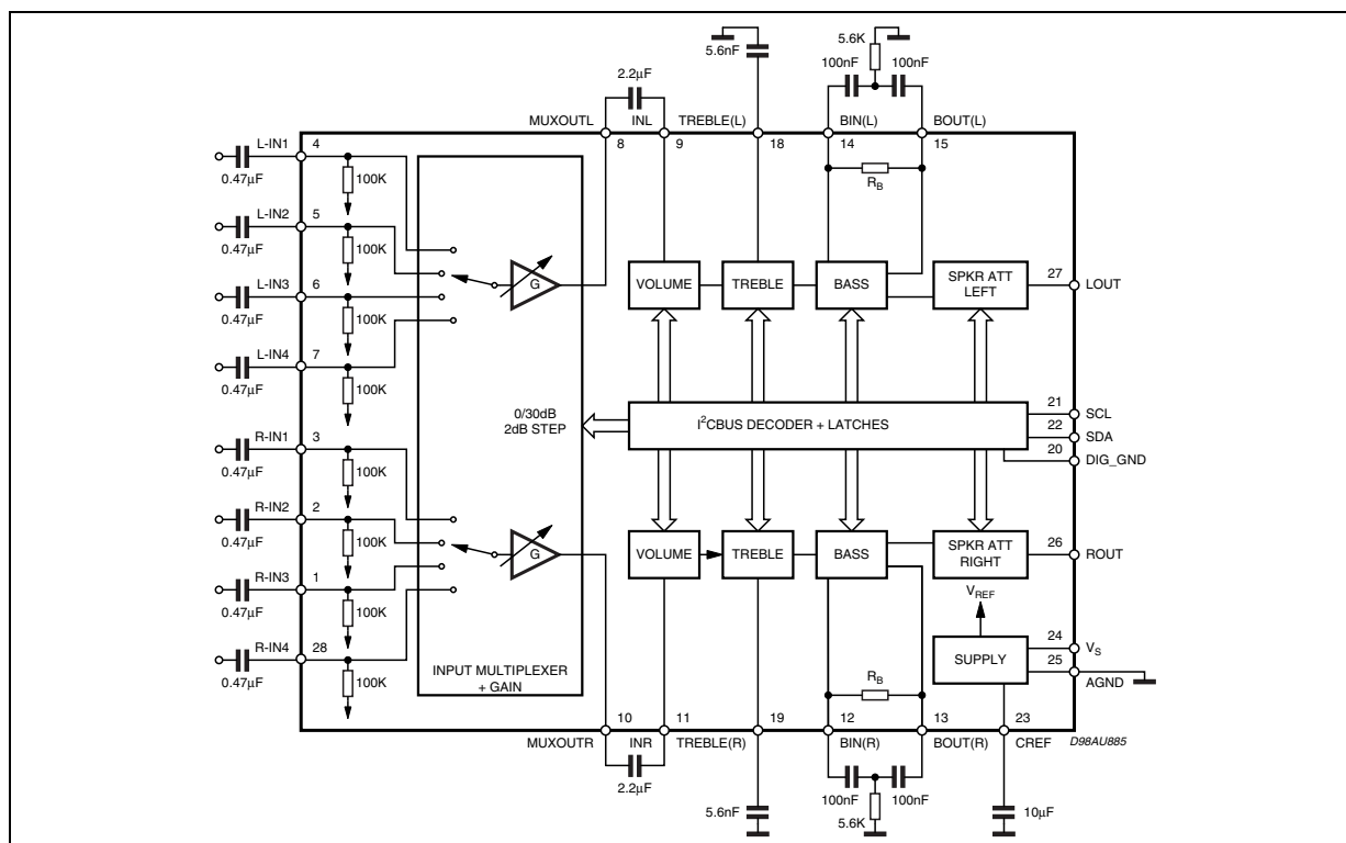
Figure 4. Test Circuit
