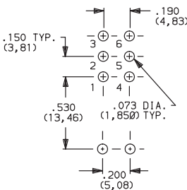
PC MOUNTING
