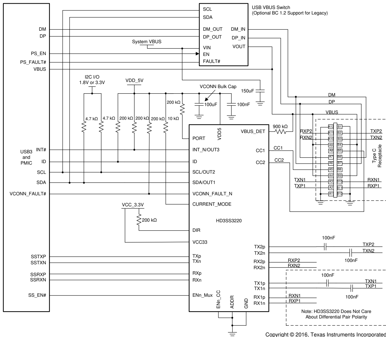
Figure 7-2. DFP Application Using HD3SS3220DFP
