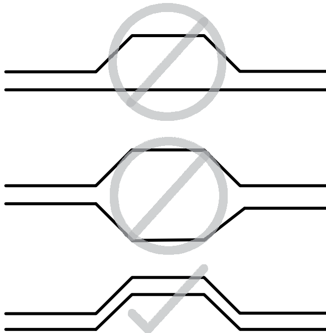
Figure 9-4. Differential Pair Symmetry
