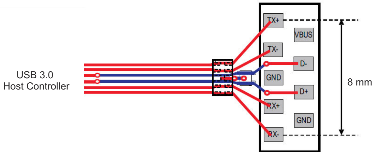
Figure 9-9. Flow-Through Routing
