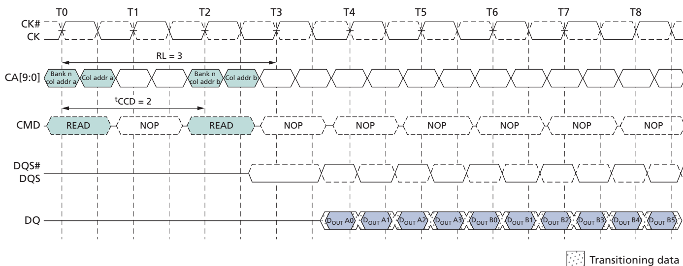
Figure 38: READ Burst Interrupt Example – RL = 3, BL = 8, t_{CCD} = 2
