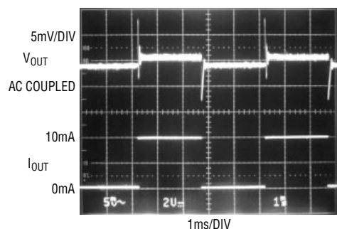
Load Transient Response (See Figure 2, V_{CC} = 5\text{V} )
