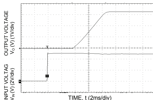
Figure 16. Typical Start-Up with application of V_{in} ( V_{in} = 5.0\text{Vdc} , V_o = 3.3\text{Vdc} , I_o = 3\text{A} ).
