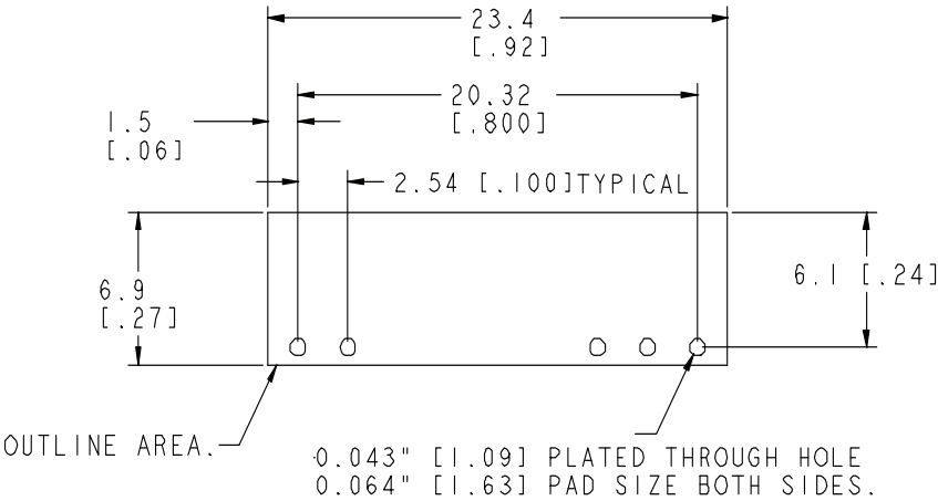
Component side view
