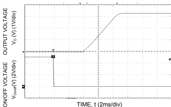
Figure 15. Typical Start-Up Using Remote On/Off with Low-ESR external capacitors ( 7 \times 150\text{ }\mu\text{F} Polymer) ( V_{in} = 5.0\text{Vdc} , V_o = 3.3\text{Vdc} , I_o = 3\text{A} , C_o = 1050\text{ }\mu\text{F} ).
