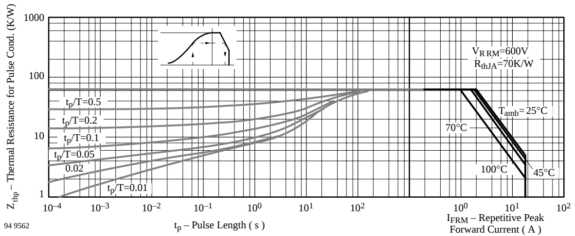
Figure 5. Thermal Response
