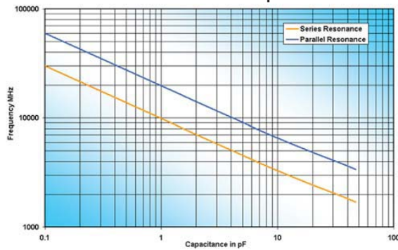
C06 Resonance vs. Capacitance
