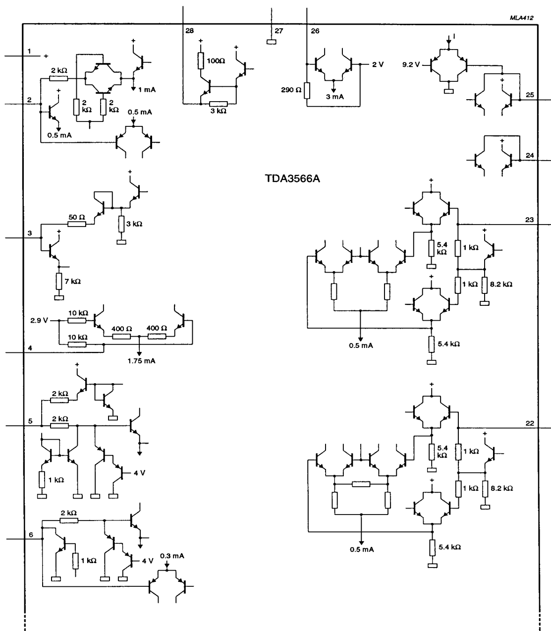
Fig.10 Internal pin circuitry (first part).
