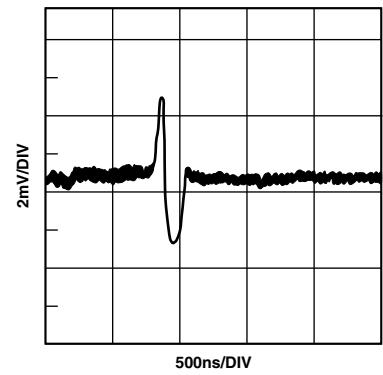
Figure 25. DAC-DAC Crosstalk
