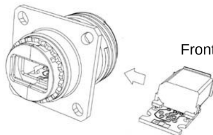
Type 2 : Solder 6 Tined holes for soldering
