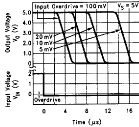
Response Time for Various Input Overdrives — t_{PHL}
