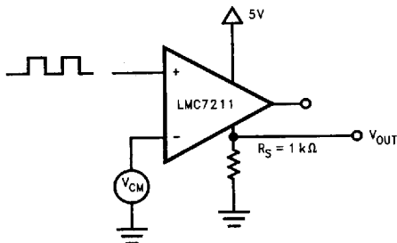
FIGURE 2. Circuit for Measurement of the Shoot-Through Current
