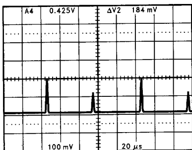
FIGURE 3. Measurement of the Shoot-Through Current
