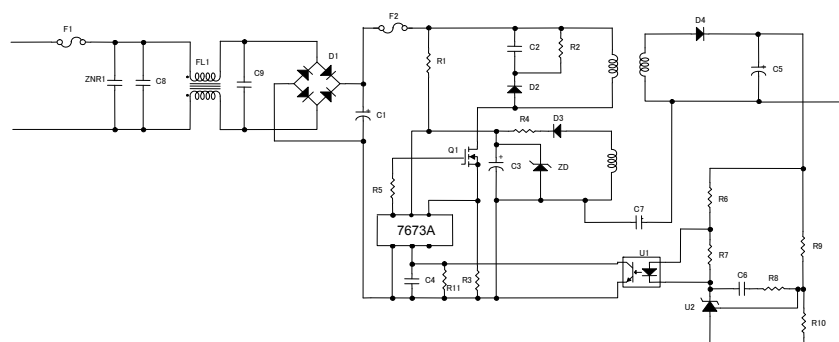
Figure 1, Application Diagram (12 V 1A Isolated Type)
