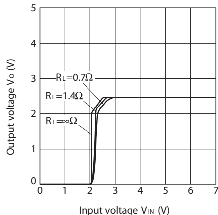
Fig.9 Output Voltage vs. Input Voltage (PQ025Y3H3ZxH)
