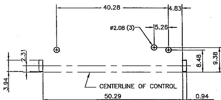
PCB LAYOUT GENERAL TOL \pm 0.05
