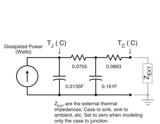
Figure 5b, TRANSIENT THERMAL IMPEDANCE MODEL
